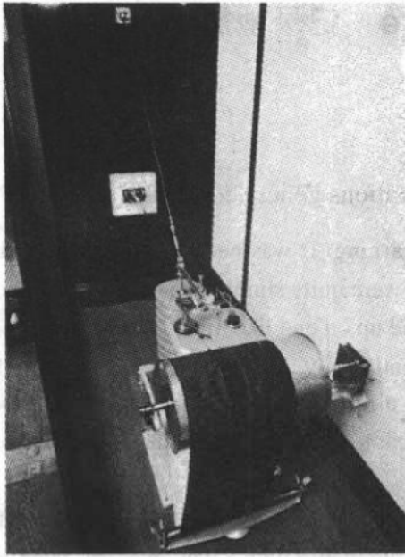
The Shaw seismograph at the Science Museum, London
